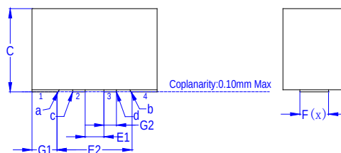
Suggested Pad Layout
