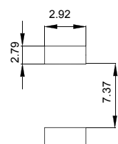
SUGGEST PCB LAYOUT
