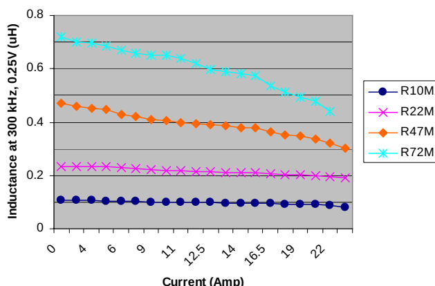
SC7232 Family DC Bias Curve (0.1~0.72 μH)
