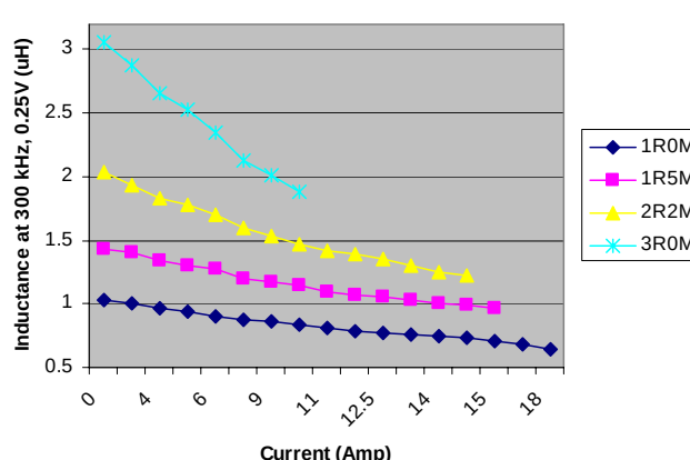
SC7232 Family DC Bias Curve (1.0~3.0 μH)
